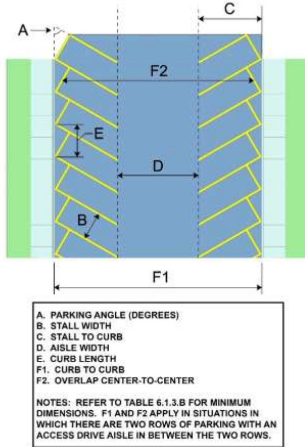
FIGURE 6.1.3.B.1: PARKING DIMENSIONS
