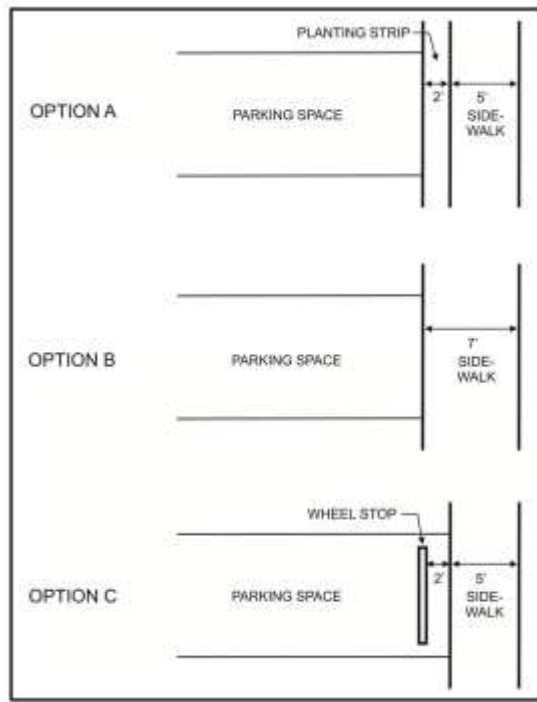
FIGURE 6.1.3.G: SIDEWALK TREATMENTS
