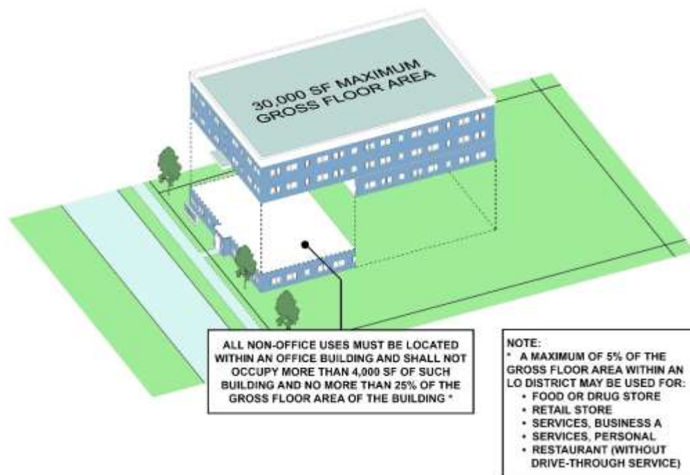
FIGURE 4.6.2.E: CERTAIN USE-BASED GROSS FLOOR AREA RESTRICTIONS – LO DISTRICT
