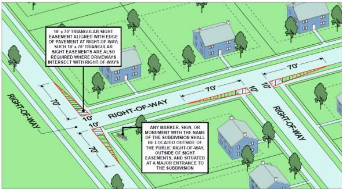
FIGURE 3.2.9.D.4: SIGHT EASEMENTS
