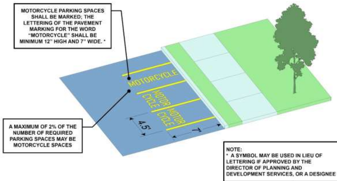
FIGURE 6.1.5.F – MOTORCYCLE PARKING SPACE REQUIREMENTS
